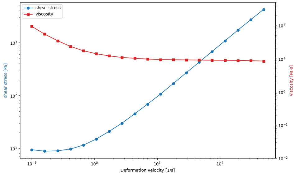
Figure 4: The graph shows the measurements of honey. On the left y-axis the shear stress and on the right y-axis the viscosity is plotted, both of these are plotted against the deformation velocity.
